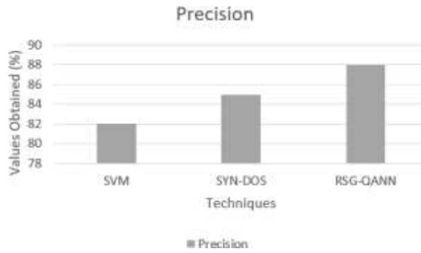
(e) precision Figure-3 Comparative for DARPA 98 dataset
