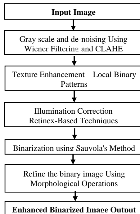
Figure 2: Flowchart illustrating the Proposed Methodology
