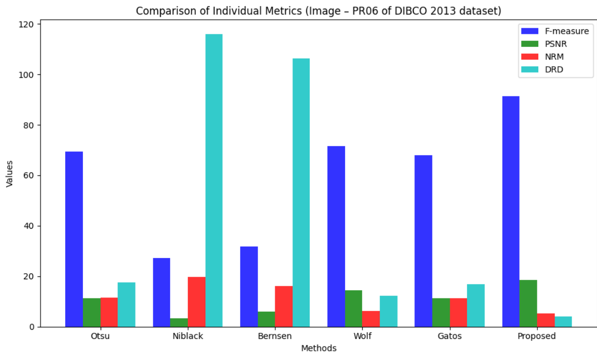
Figure 6: graph plot for Table-1 of Image – PR06 of DIBCO 2013 dataset (figure 4)
