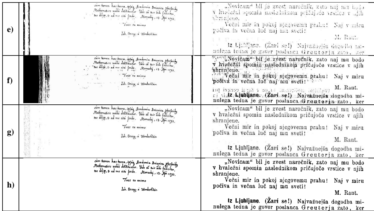
Figure 4: Evaluation of results from our proposed method compared to other methods: a) Input image, b) Otsu's result, c) Niblack's result, d) Bernsen's result, e) Wolf's result, f) Gatos's result, g) Proposed method's result, h) Ground truth image.
