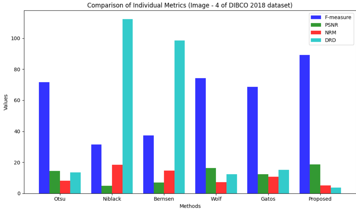
Figure 5: graph plot for Table-1 of Image - 4 of DIBCO 2018 dataset (figure 4)
