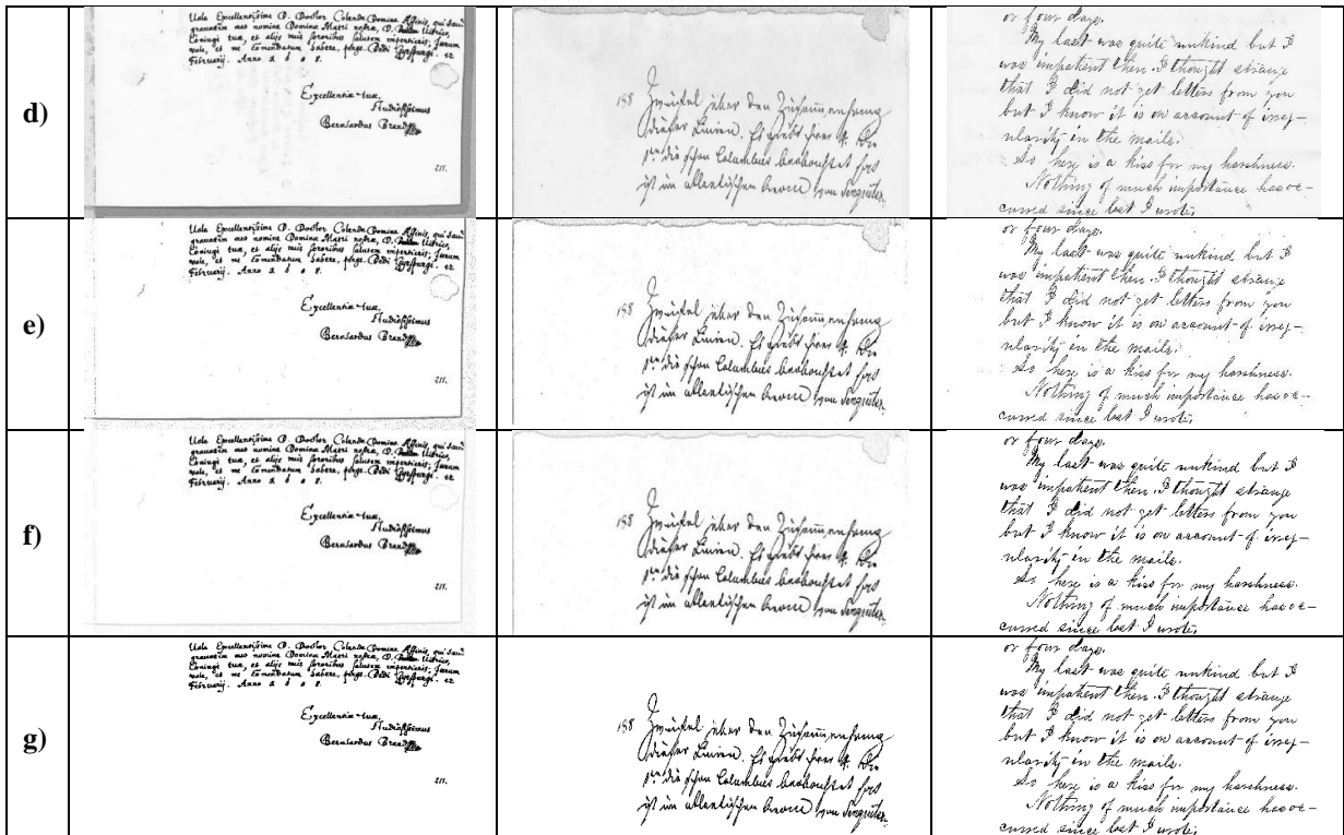
Figure 3: Illustrates the results of proposed method in each stages: a) The input image. b) The output after preprocessing. c) The image after texture enhancement. d) The result of illumination correction. e) The outcome of Sauvola. f) The final result after post-processing using morphological opening operation. g) ground truth image.
