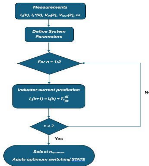
Fig. 7. Flowchart of the MPC algorithm
