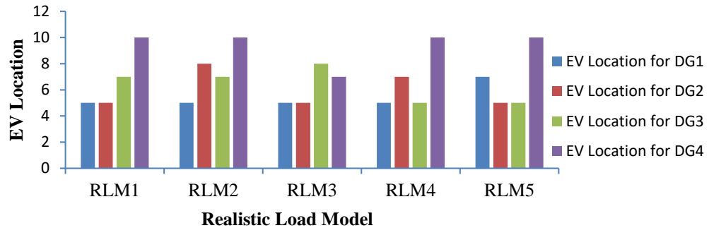
Fig.6: Comparison of various optimal EV location profile of 16-bus system for RLMs
