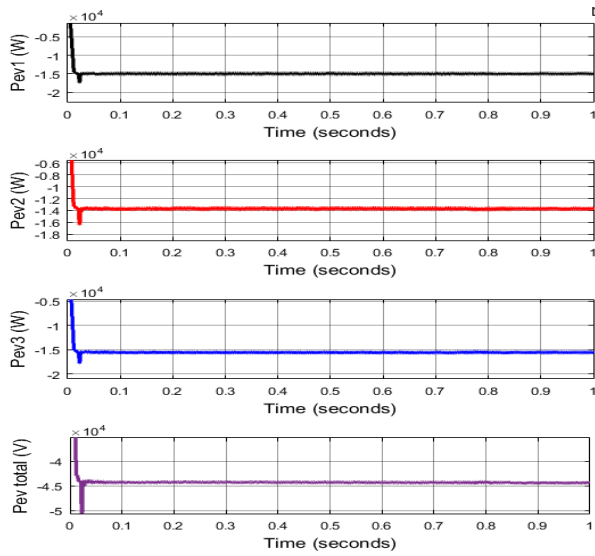
Figure 11: Active powers of EVs during G2V mode
