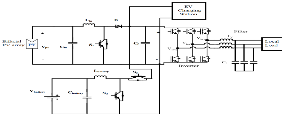
Figure 2: Circuit structure of standalone PV source with battery backup storage
