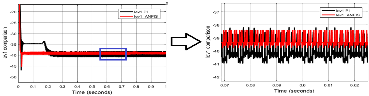
Figure 16: EV battery current comparison during G2V mode
