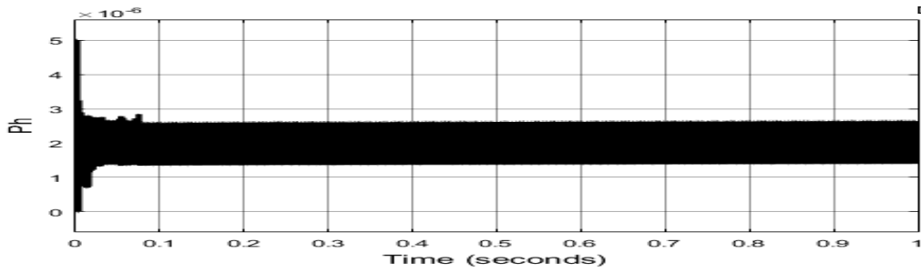
Figure 15: Phase delay time of DC common link connected full bridge during V2G mode
