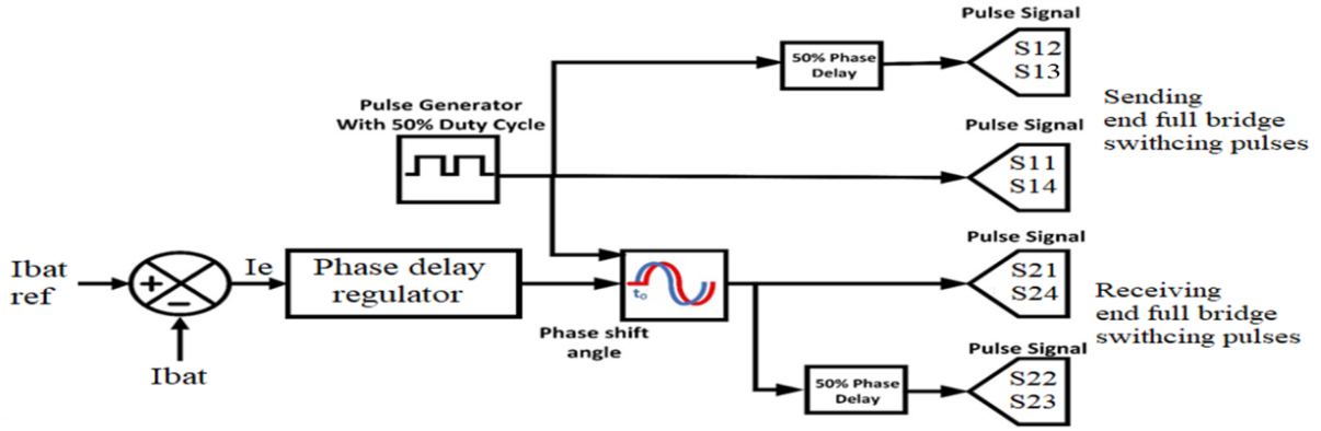
Figure 5: Phase delay regulator controller of MAFB circuit
