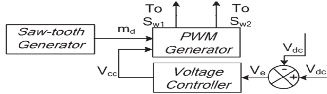
Figure 3: Voltage regulator controller
