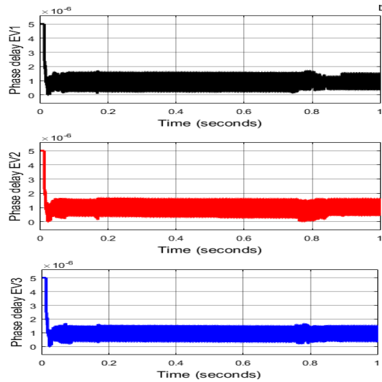
Fig 12: Phase delay time of EV full bridges switches during G2V mode
