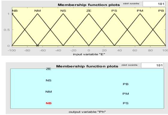
Figure 6: ANFIS variable MFs
