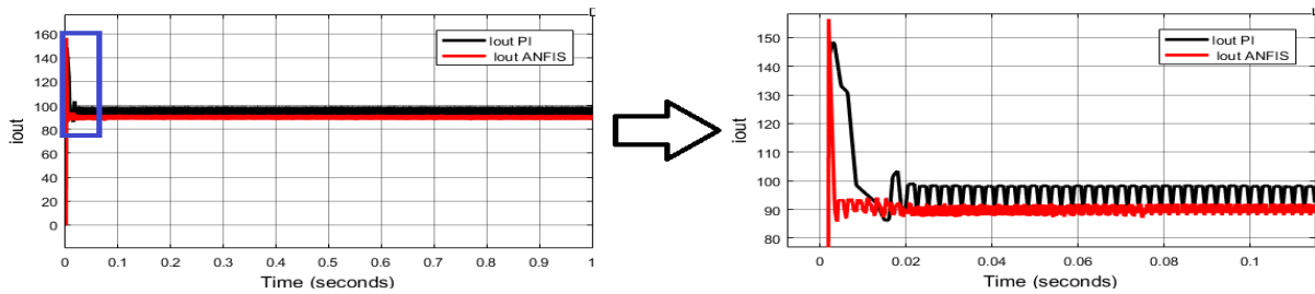
Figure 17: DC common link side full bridge output current comparison during V2G mode
