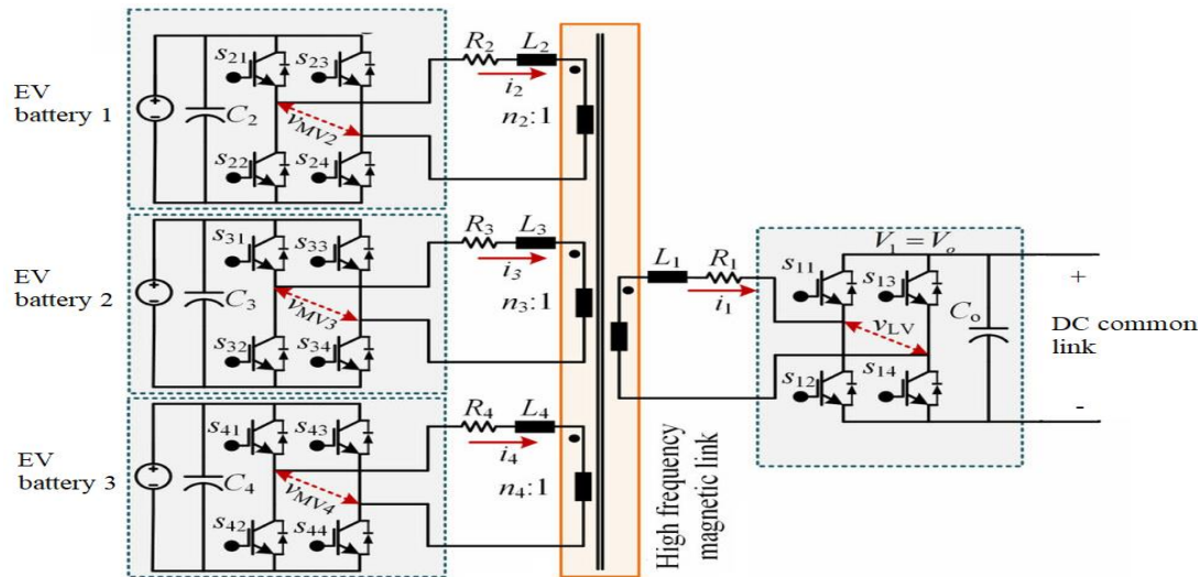
Figure 4: MAFB circuit topology for EV charging station
