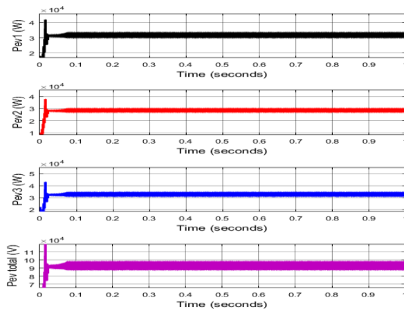
Figure 14: Active powers of EVs during V2G mode
