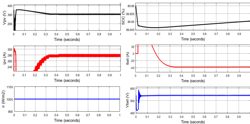
Figure 8: Bifacial PV array characteristics
