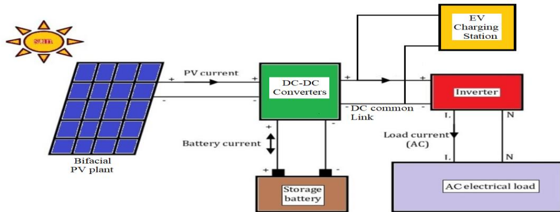
Figure 1: Outline structure of standalone PV plant with EV charging station
