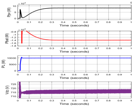
Fig 13: Active powers of Bifacial PV array, battery, load and DC common voltage during V2G
